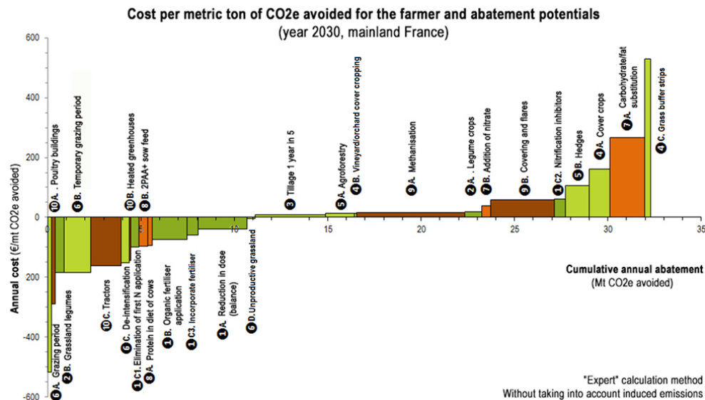
Figure 1. Example MACC curve, showing cost per tonne of CO 2 e avoided for the farmer and abatement potential for France. Source: Pellerin et al. (2013).
