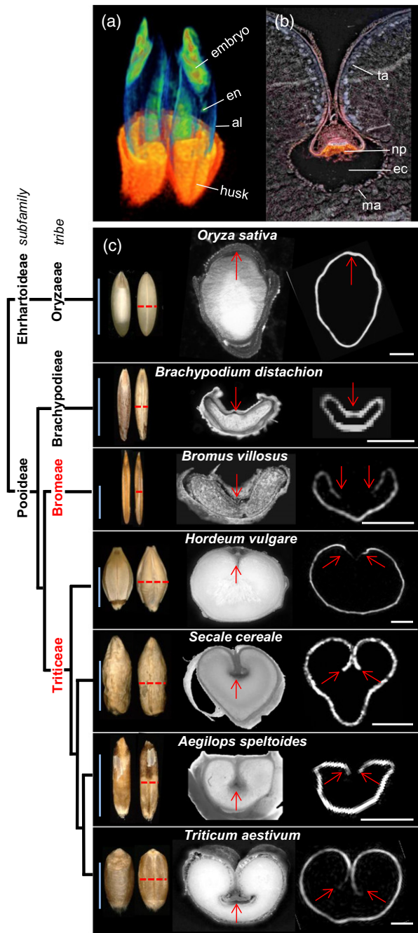
Figure 6. Nuclear magnetic resonance imaging of the grains of the representative species from Triticeae, Bromoideae, Brachypodioideae and Oryzoideae tribes.
