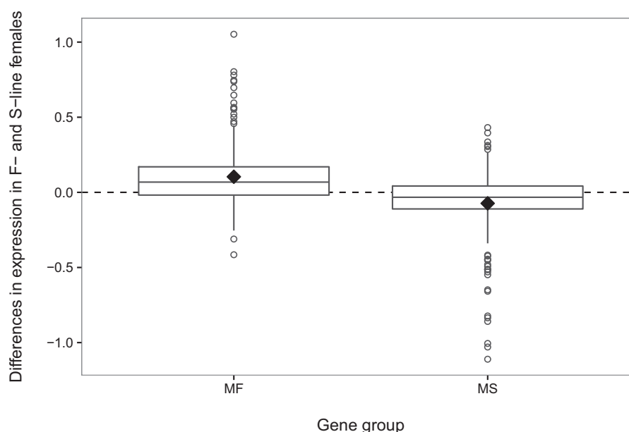
Fig. 1. —Boxplot for differences in expression between F-line and S-line females for genes biased in males (positive difference represents higher expression in F-line females). Y-axis depicts difference in mean over replicate lines for log transformed expression values (FPKM) in F-line and S-line females. Diamonds represent means. F-male-biased genes (MF), S-male-biased genes (MS).
