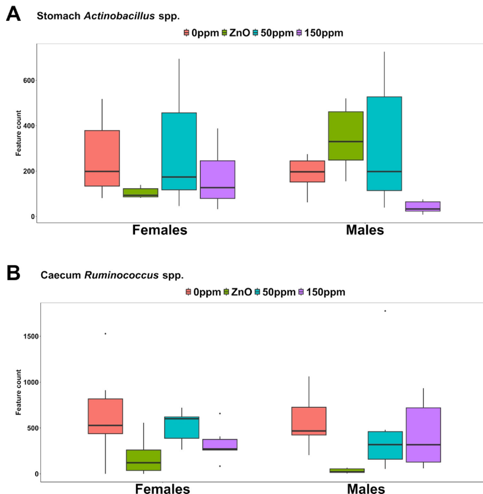
Fig. 1. Feature count of Actinobacillus spp. In the stomach (A) and Ruminococcus spp. In the caecum in males and females through the different treatments.
